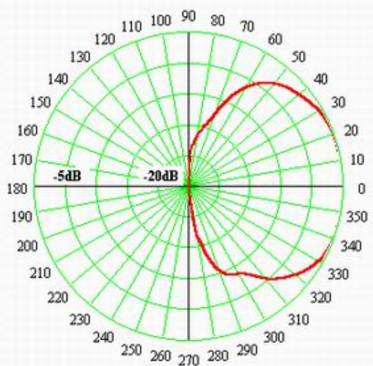
Radiation Pattern PA5.9 SA in H-plane
